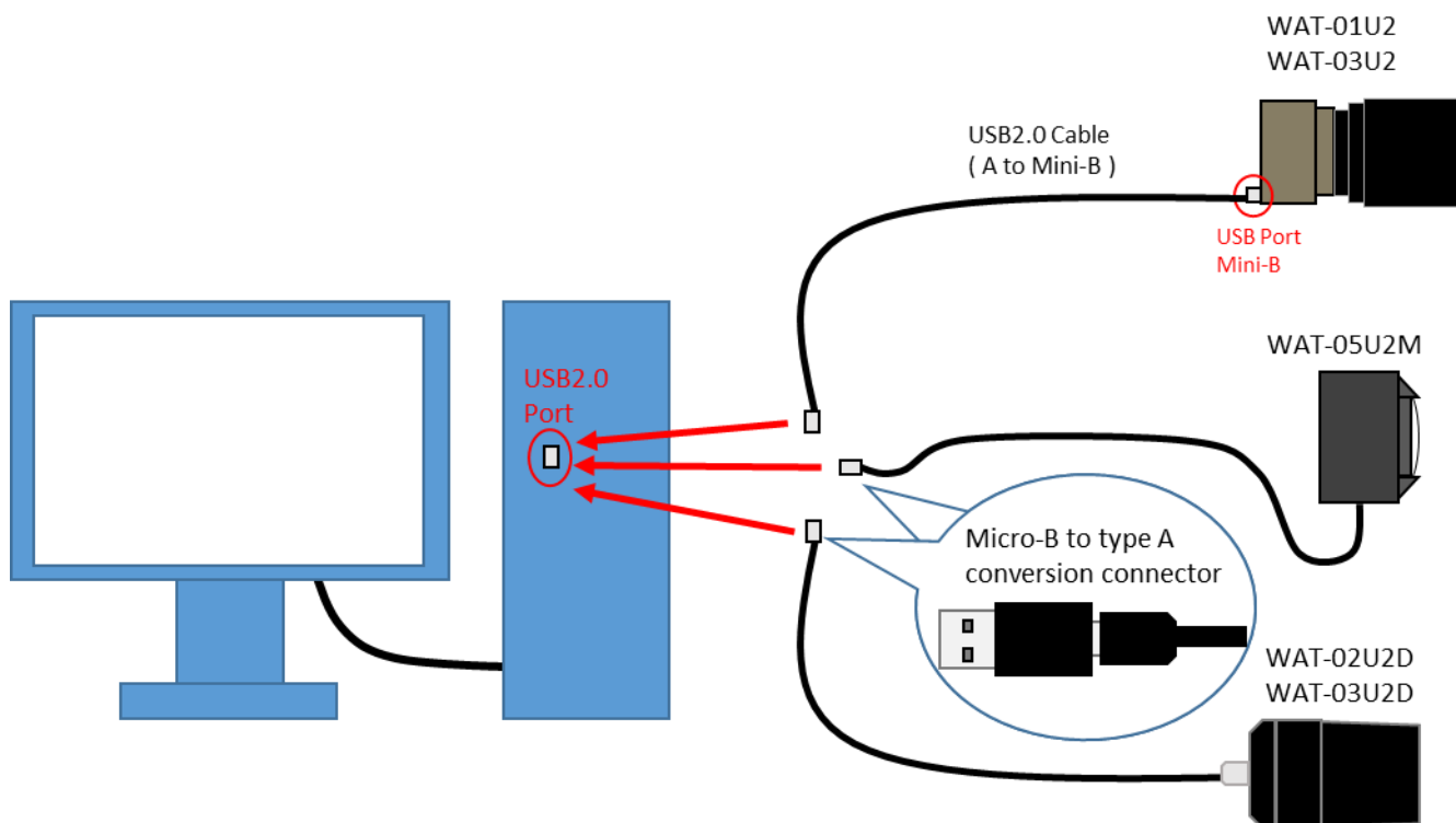
Fig.1 Watec USB Camera - PC Connection Diagram
